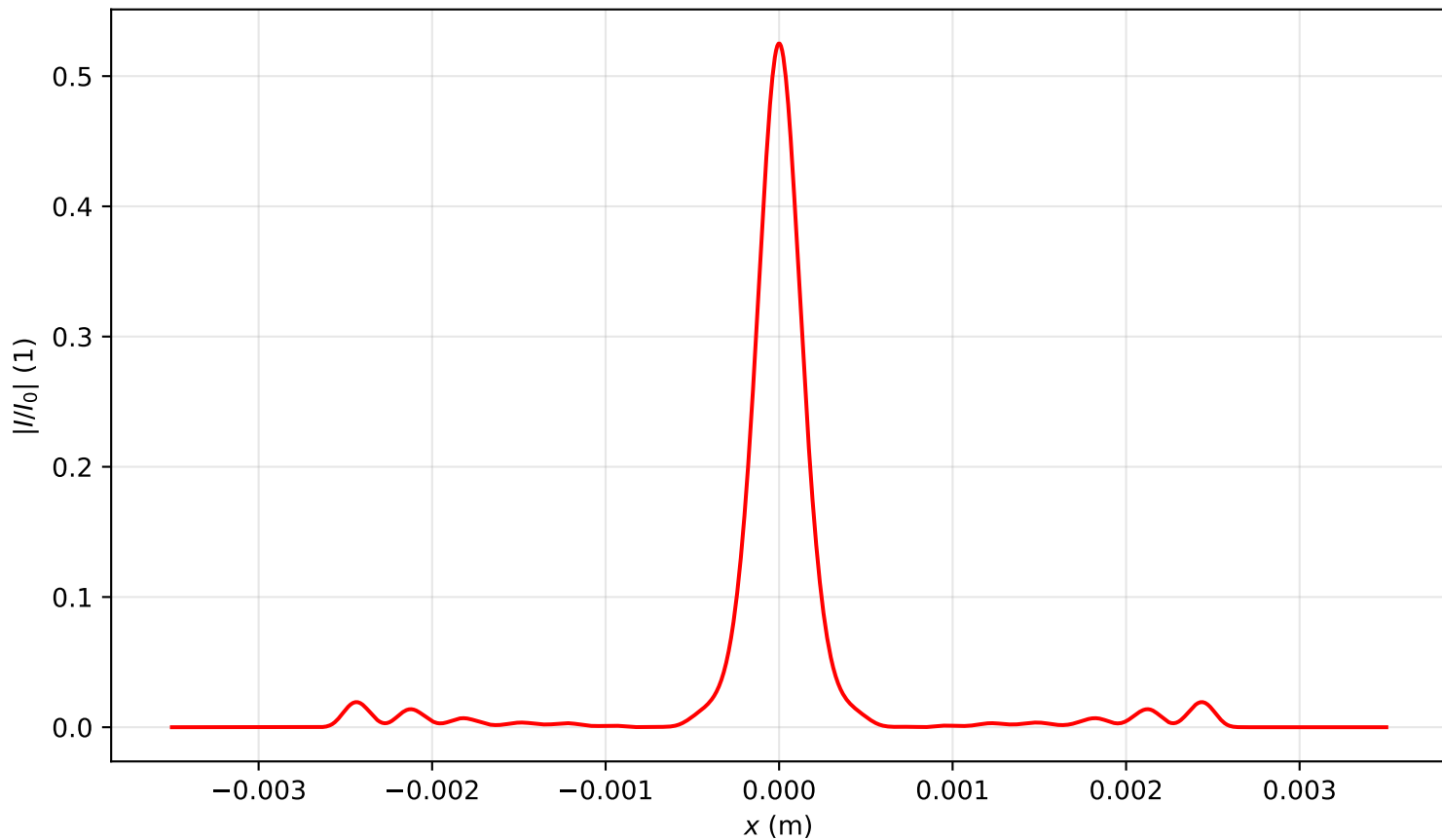
Intensity profile I(x, y = 0, z = 2.070)/I_0 , \text{Pin}=7.0\text{Pcr} , artificial time
